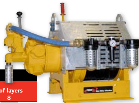
FA2i-MR12MK1G with Optional Air Preparation Package
